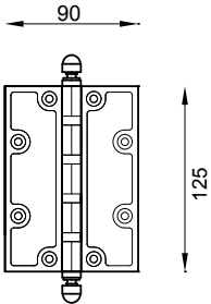
2307/1 cerniera Classic Classic hinge
