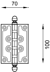
2307 cerniera Classic Classic hinge
