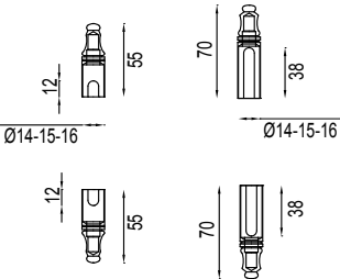
2313 set copricerniere corto con piramide short cover hinges set with pyramid
